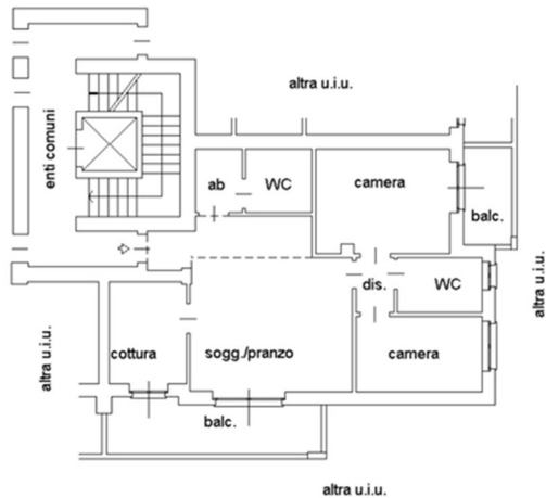
PIANO TERZO H=2.70m
