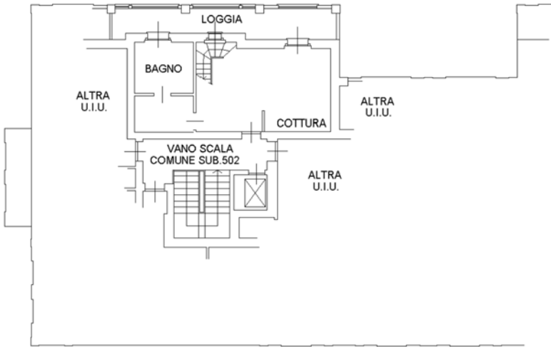
PIANO TERZO H=2.70
