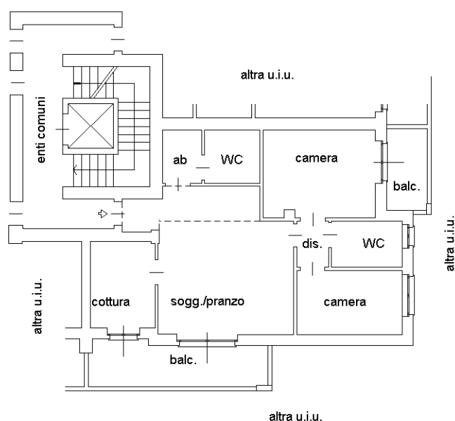
PIANO TERZO H=2.70m
